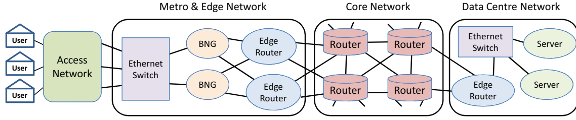
Figure 5.1: Topology of the network between a end-user and the Cloud data center.
